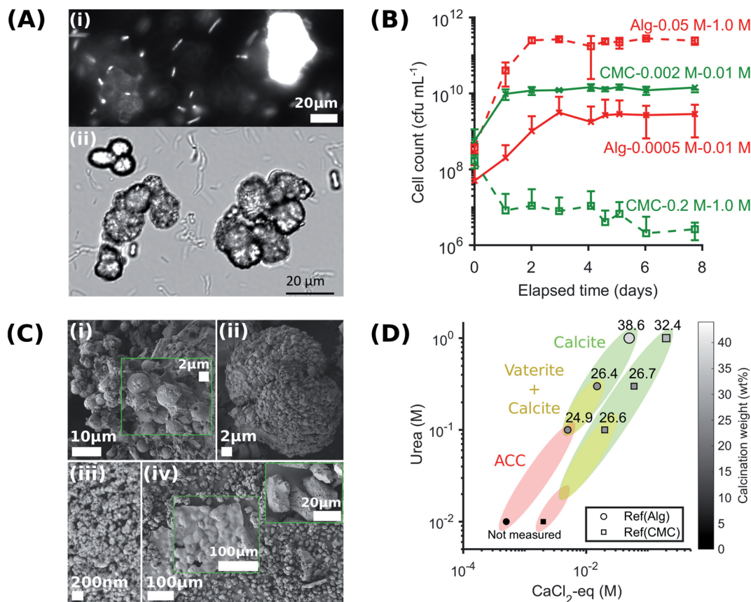
Fig. 3 Viability of S. pasteurii after release from the hydrogels, and structure and yield of \text{CaCO}_3 formed in the absence of hydrogels. (A) Observations by epifluorescence (i) and brightfield (ii) optical microscopy of bacteria and \text{CaCO}_3 precipitation in their microenvironment, respectively; (B) flow cytometry measurements of bacteria release from the hydrogel; (C) SEM-SE2 images of vaterite spherulites in Ref(Alg)-0.015 M-0.3 M (i) and amorphous calcium carbonate nano-aggregates in Ref(CMC)-0.002 M-0.01 M (iii), and calcite with rhombohedral morphology in Ref(Alg)-0.05 M-1.0 M (ii) and Ref(CMC)-0.2 M-1.0 M (iv); and (D) \text{CaCO}_3 phase diagram and yield (the symbol size and colour are proportional to the calcination weight loss).
